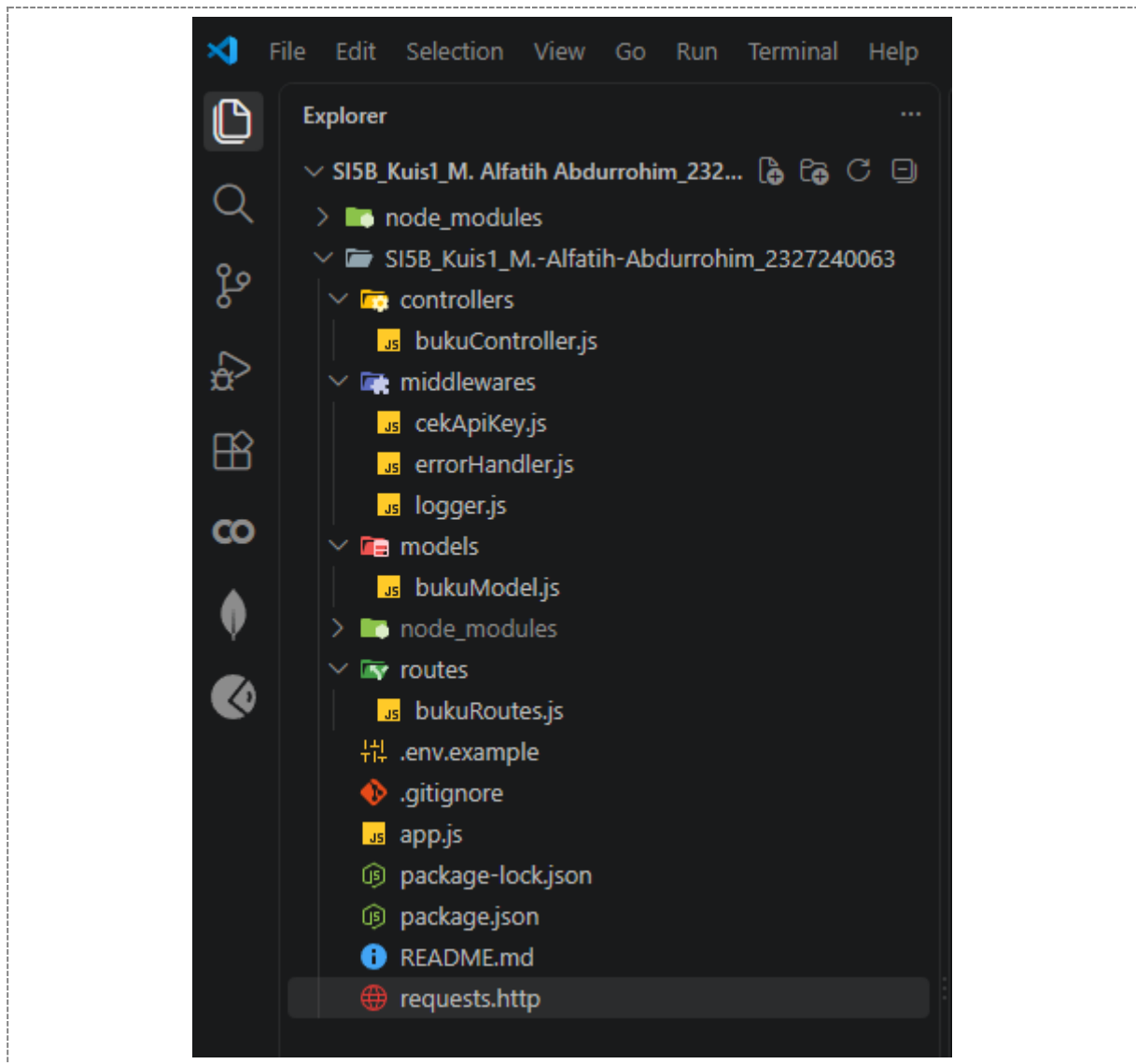
Gambar 2. Struktur folder project
